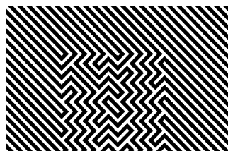
Similarity Summations
